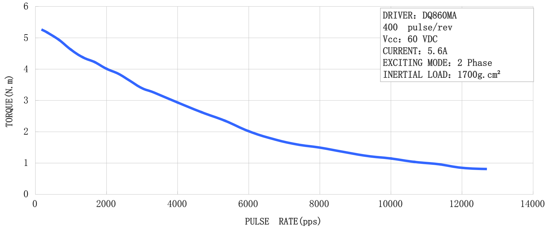
85BYGH450D-008 Torque Curve
